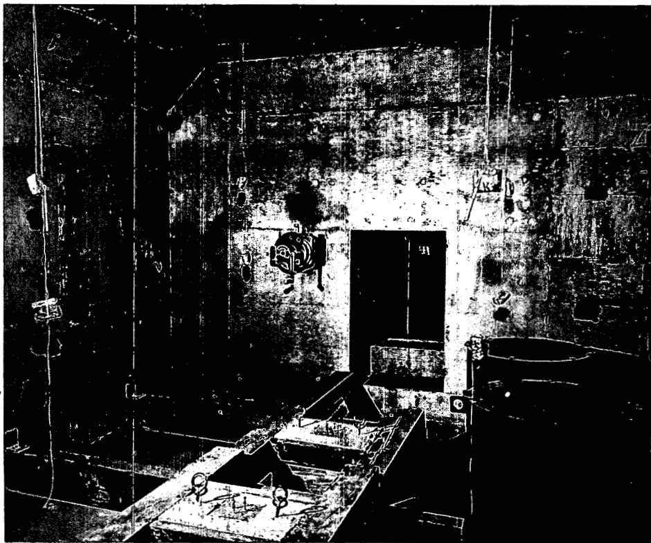
Fig. 13—Shock-gauge canisters and Ensolite test equipment.
